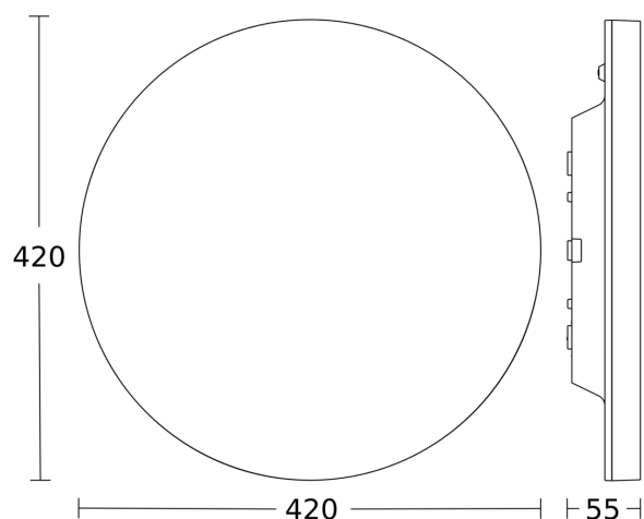
Dimension Drawing
